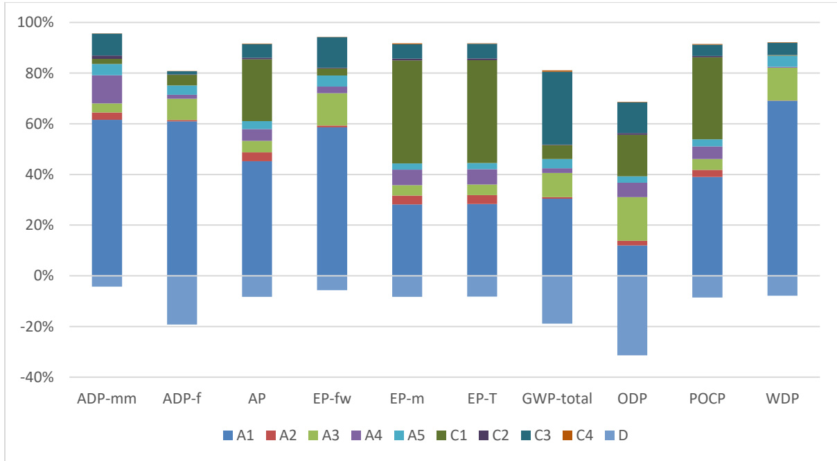
Figure 2: Tensor® TriAx® TX5 - Impact of the individual modules on the environmental core indicators
