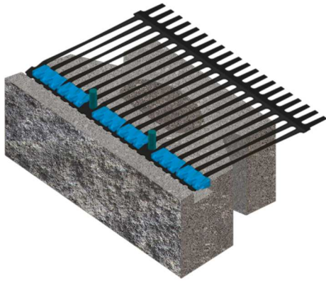
Figure 2. Keystone TW3 modular block retaining wall system
