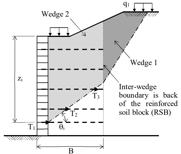
Figure 3. Basis of the two-part wedge method
