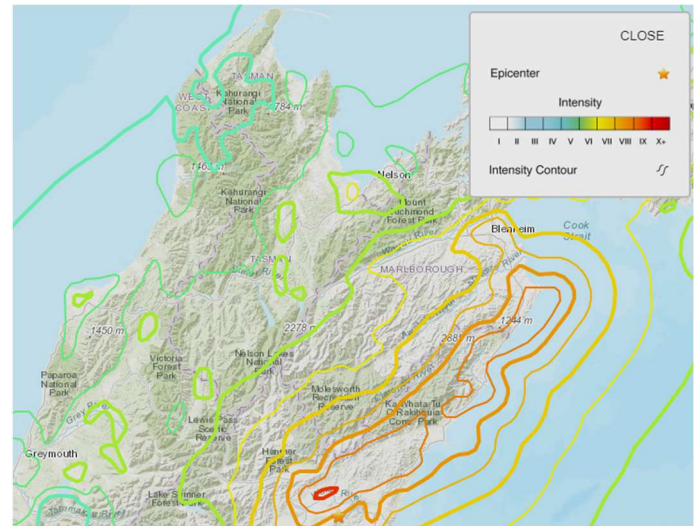
Figure 9. USGS ShakeMap for the M_w = 7.8 Kaikoura earthquake showing intensity contours (Source: United States Geological Survey – USGS)
