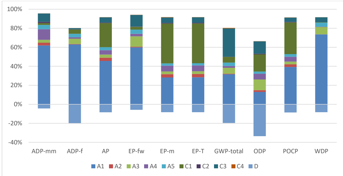
Figure 2: Tensor® TriAx® TX150 - Impact of the individual modules on the environmental core indicators
